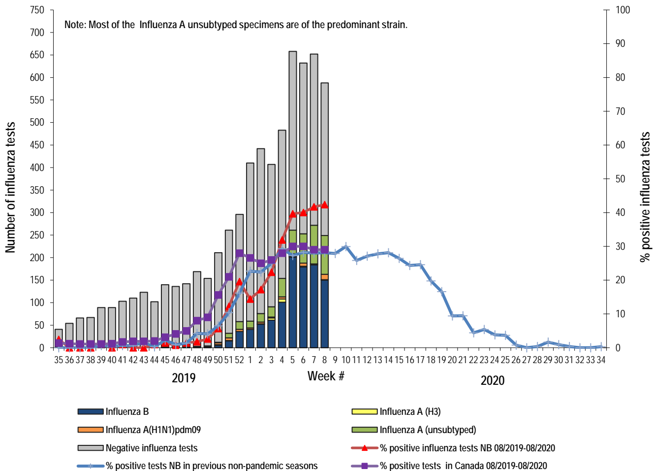
Graph 1: Number and percent of positive influenza specimens 2 in New Brunswick by week, up to February 22, 2020 (data source: G. Dumont Lab results)
